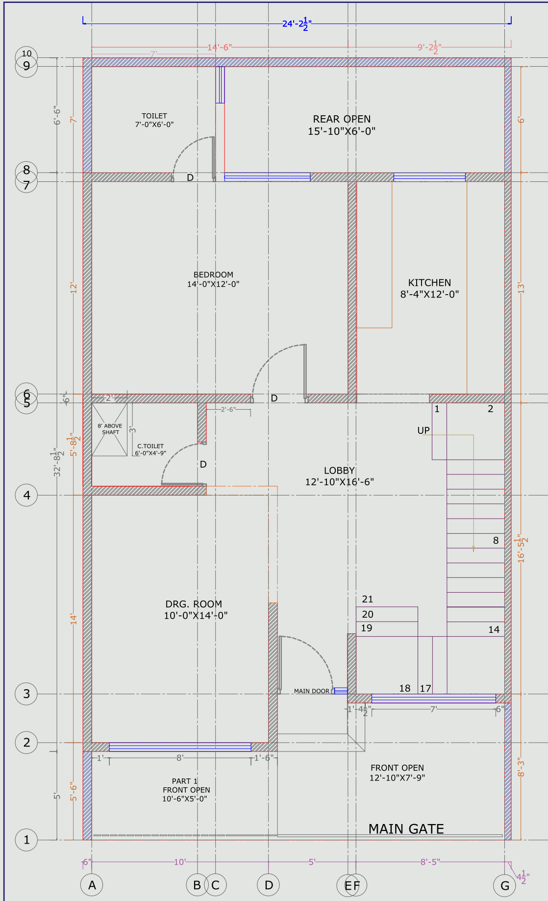
Ground Floor (32, 40, 41, 42, 43)
