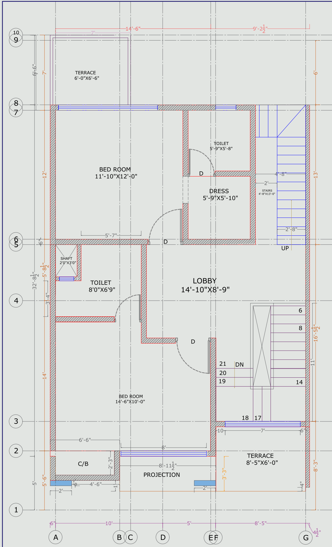
First Floor (32, 40, 41, 42, 43)
